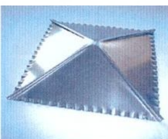
Art. B20 Fe Zn 345 x 345 mm H 60 mm
