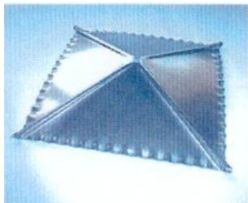
Art. B21 Fe Zn 305 x 305 mm H 60 mm
